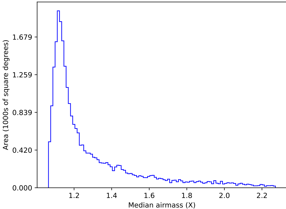
weather_cloudso18v3.4_10yrs Yr 1 i band: Median airmass
