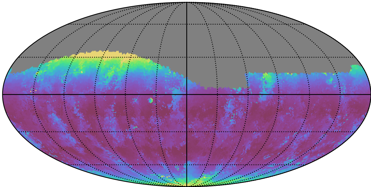
weather_cloudso18v3.4_10yrs Yr 1 g band: Median airmass
