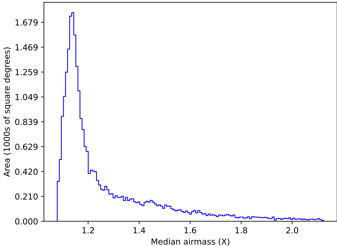
weather_cloudso18v3.4_10yrs Yr 1 all bands: Median airmass
