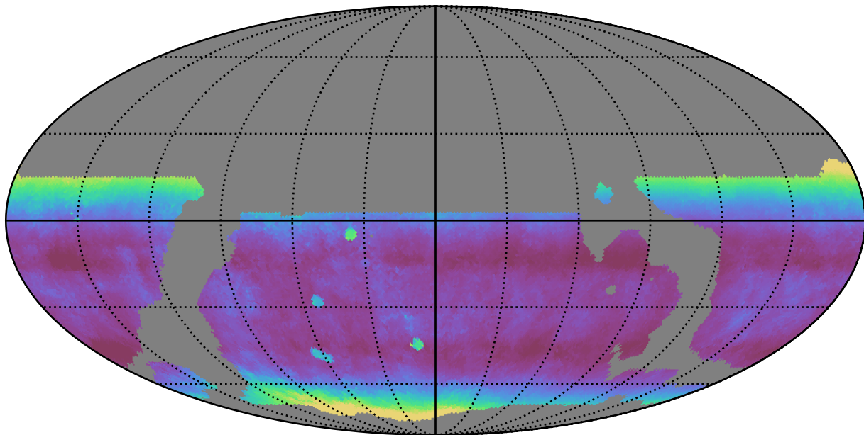
weather_cloudso18v3.4_10yrs WFD z band: Median airmass
