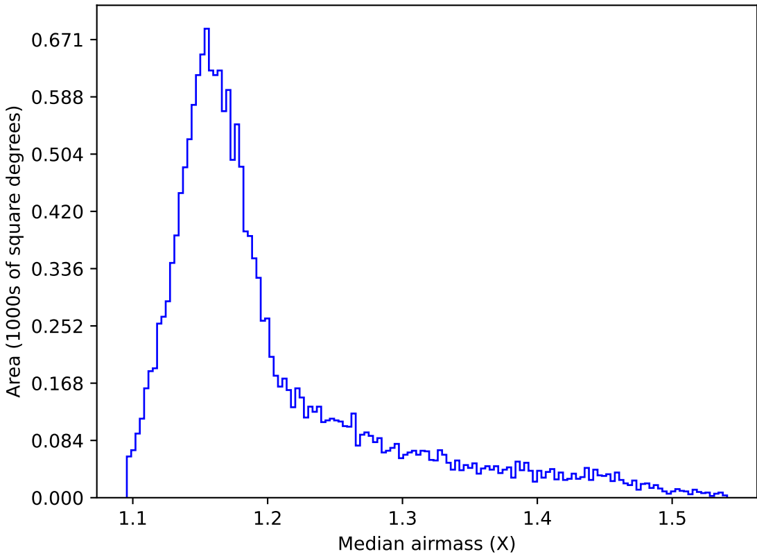
weather_cloudso18v3.4_10yrs WFD z band: Median airmass
