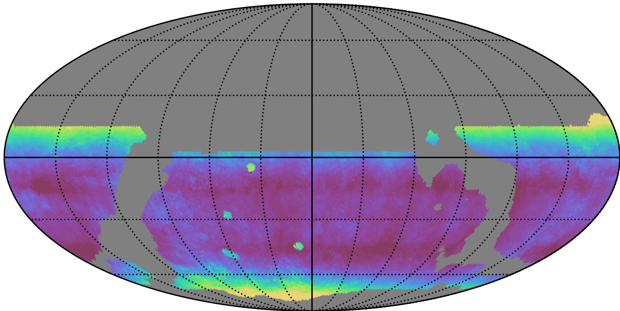
weather_cloudso18v3.4_10yrs WFD y band: Median airmass
