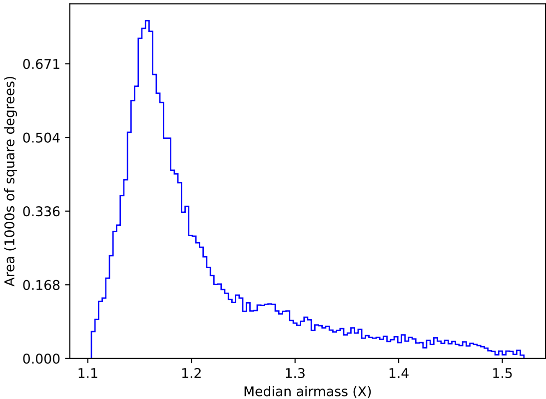
weather_cloudso18v3.4_10yrs WFD y band: Median airmass
