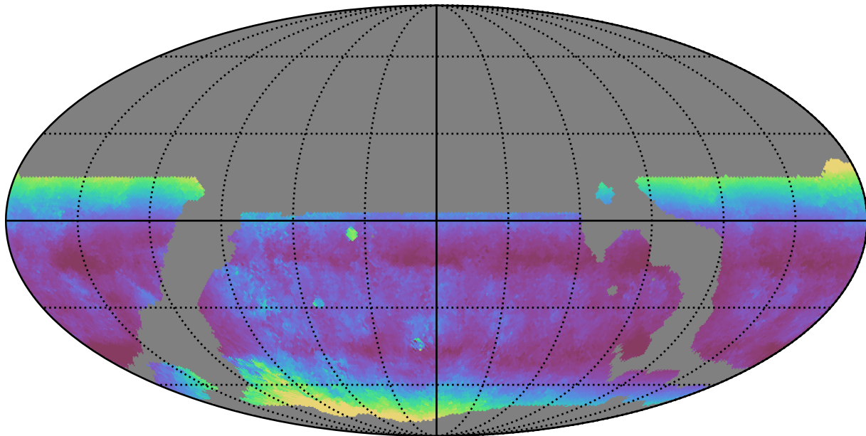
weather_cloudso18v3.4_10yrs WFD u band: Median airmass
