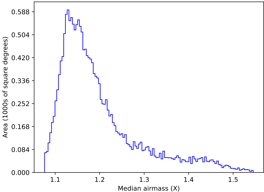
weather_cloudso18v3.4_10yrs WFD u band: Median airmass
