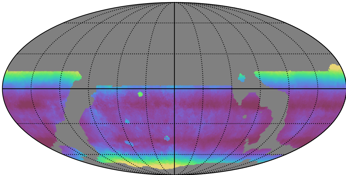
weather_cloudso18v3.4_10yrs WFD r band: Median airmass
