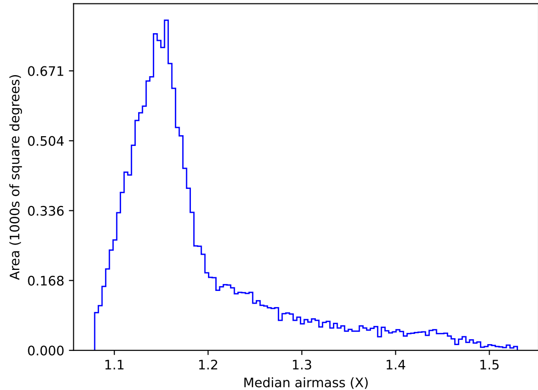
weather_cloudso18v3.4_10yrs WFD r band: Median airmass
