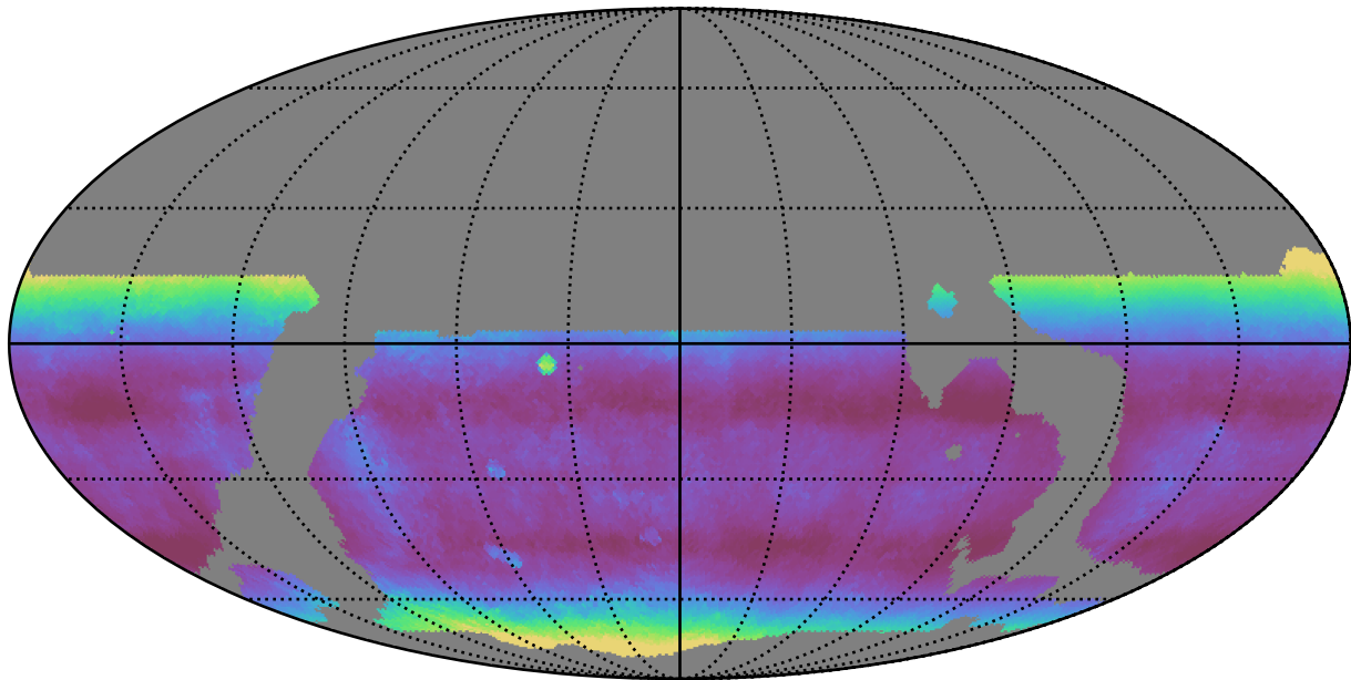
weather_cloudso18v3.4_10yrs WFD i band: Median airmass
