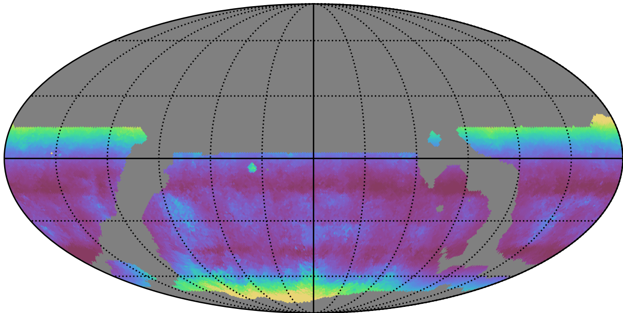
weather_cloudso18v3.4_10yrs WFD g band: Median airmass
