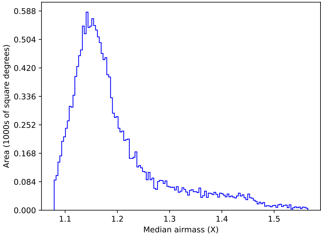
weather_cloudso18v3.4_10yrs WFD g band: Median airmass
