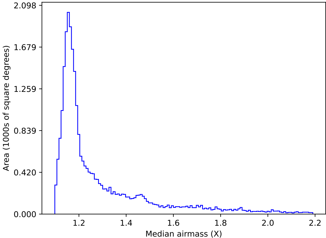
weather_cloudso18v3.4_10yrs All sky z band: Median airmass
