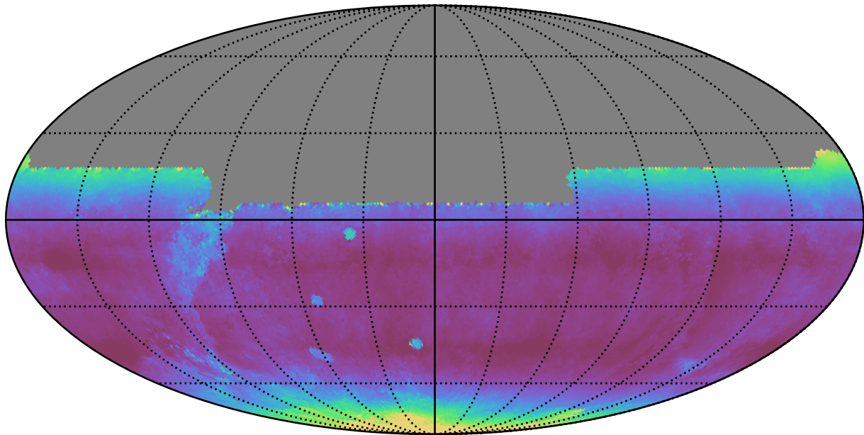
weather_cloudso18v3.4_10yrs All sky y band: Median airmass
