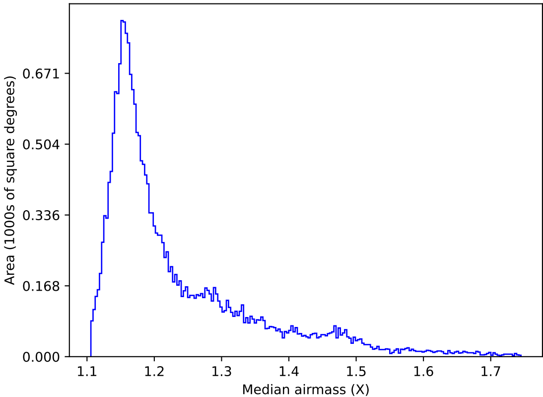
weather_cloudso18v3.4_10yrs All sky y band: Median airmass
