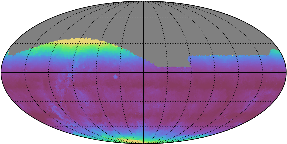
weather_cloudso18v3.4_10yrs All sky g band: Median airmass
