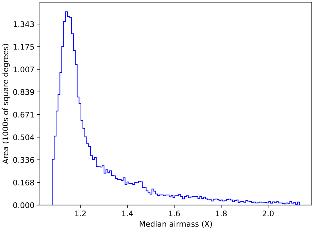
weather_cloudso18v3.4_10yrs All sky g band: Median airmass
