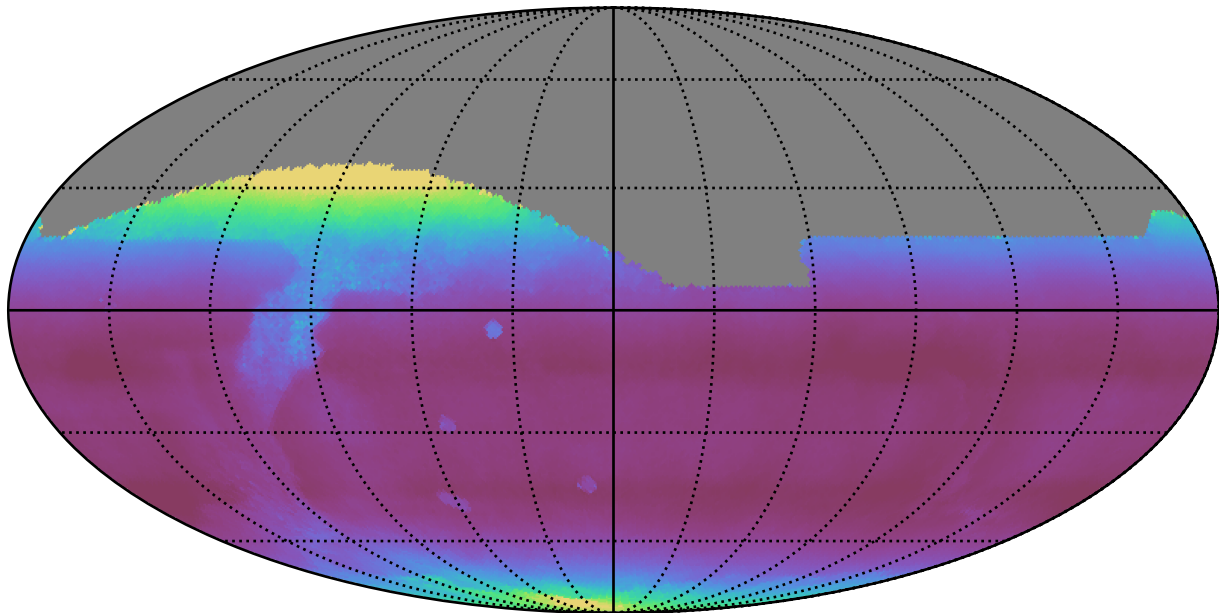
weather_cloudso18v3.4_10yrs All sky all bands: Median airmass
