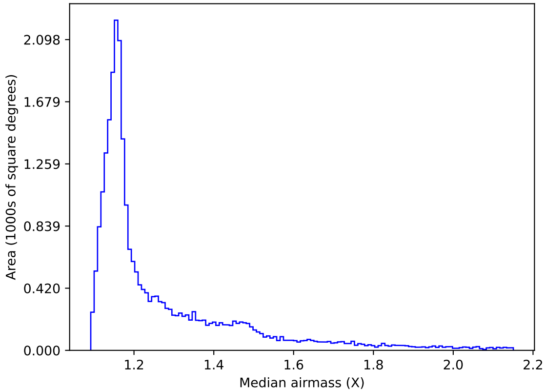
weather_cloudso18v3.4_10yrs All sky all bands: Median airmass
