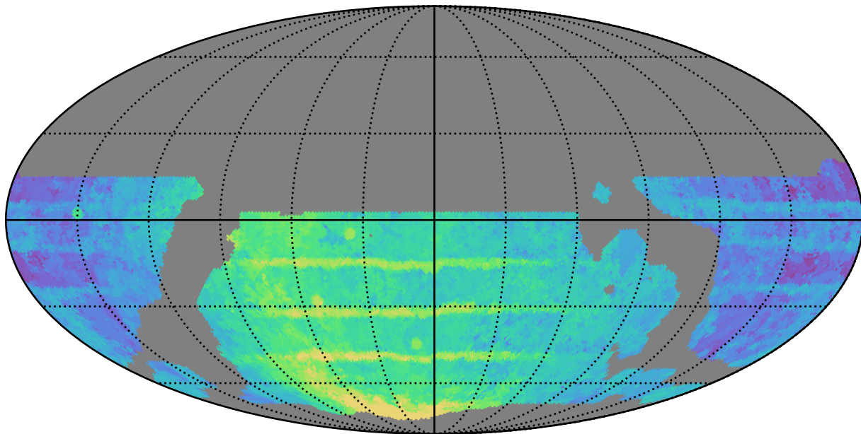
weather_cloudso18v3.4_10yrs WFD z band: Median Season Length
