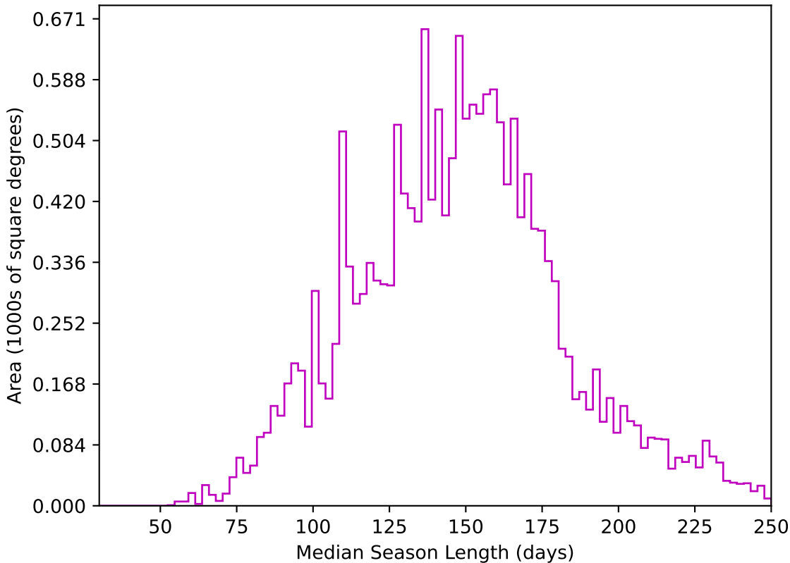
weather_cloudso18v3.4_10yrs WFD z band: Median Season Length
