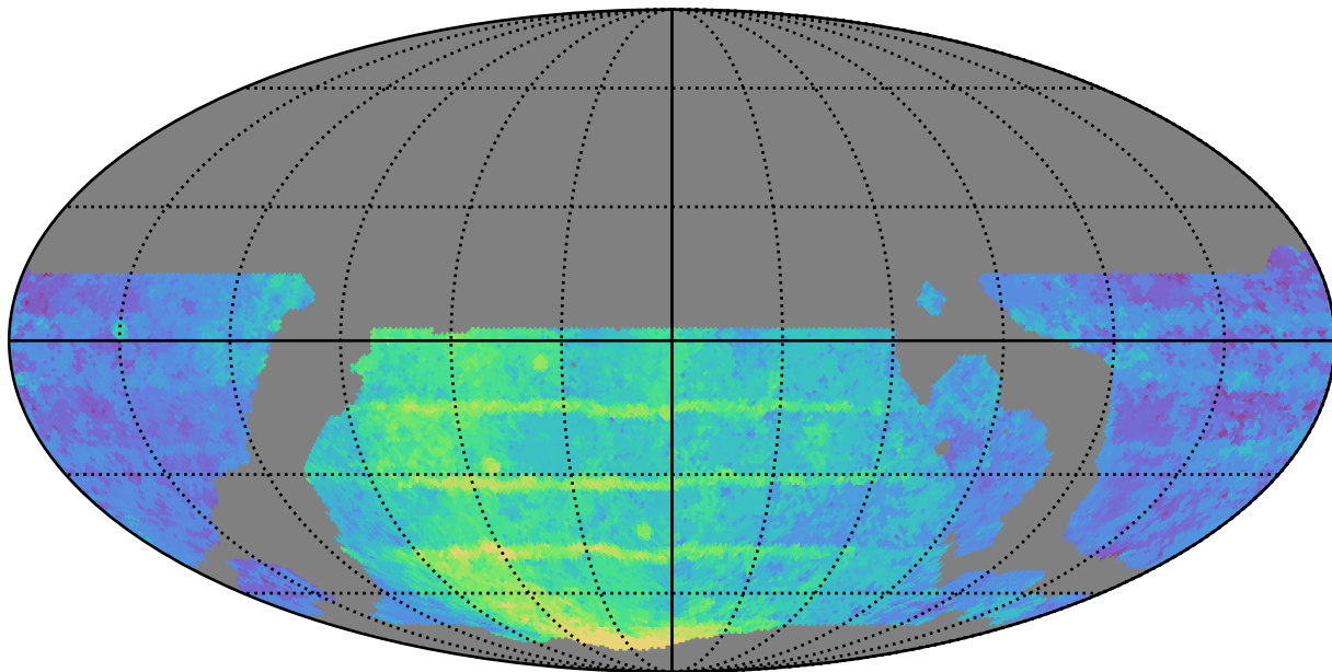
weather_cloudso18v3.4_10yrs WFD y band: Median Season Length
