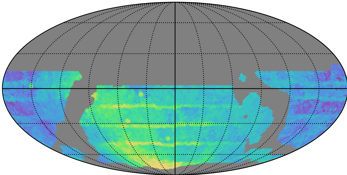
weather_cloudso18v3.4_10yrs WFD r band: Median Season Length
