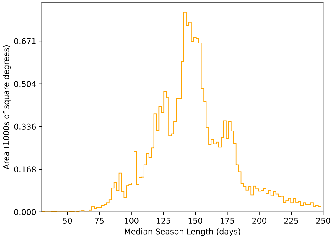
weather_cloudso18v3.4_10yrs WFD r band: Median Season Length
