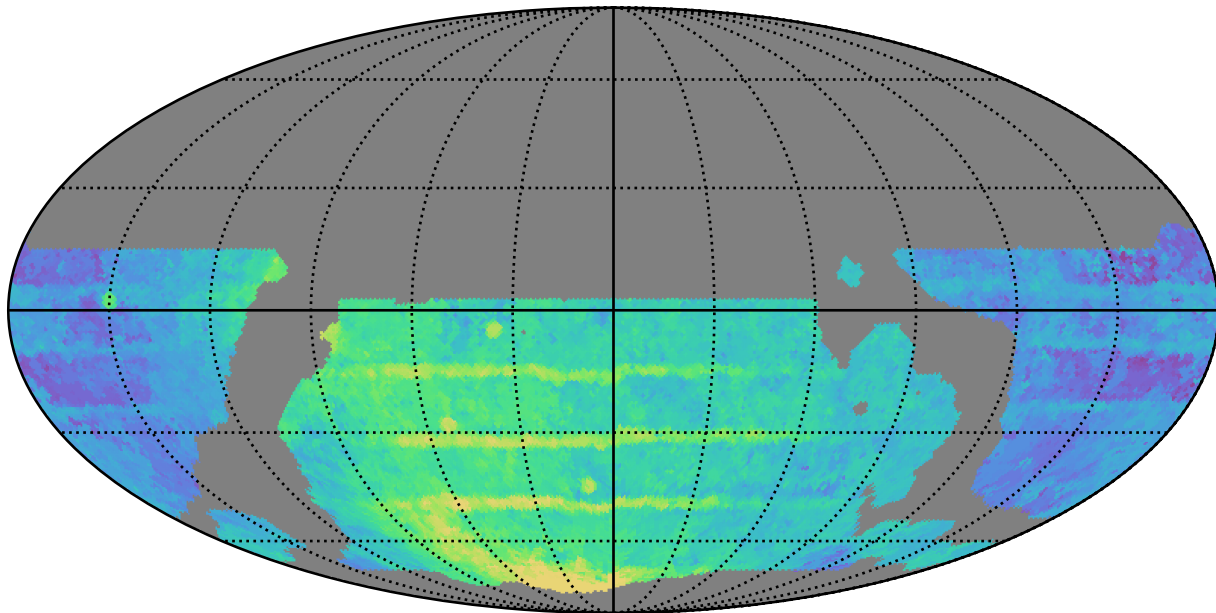
weather_cloudso18v3.4_10yrs WFD i band: Median Season Length
