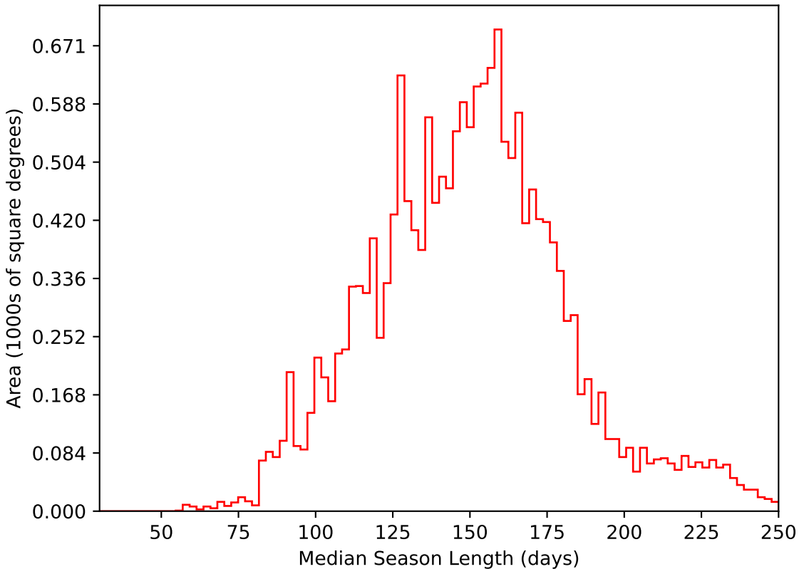
weather_cloudso18v3.4_10yrs WFD i band: Median Season Length
