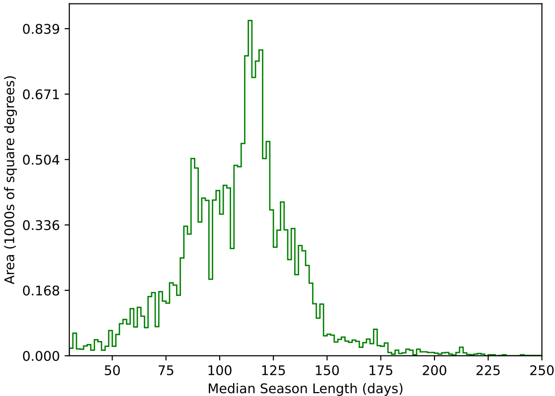
weather_cloudso18v3.4_10yrs WFD g band: Median Season Length
