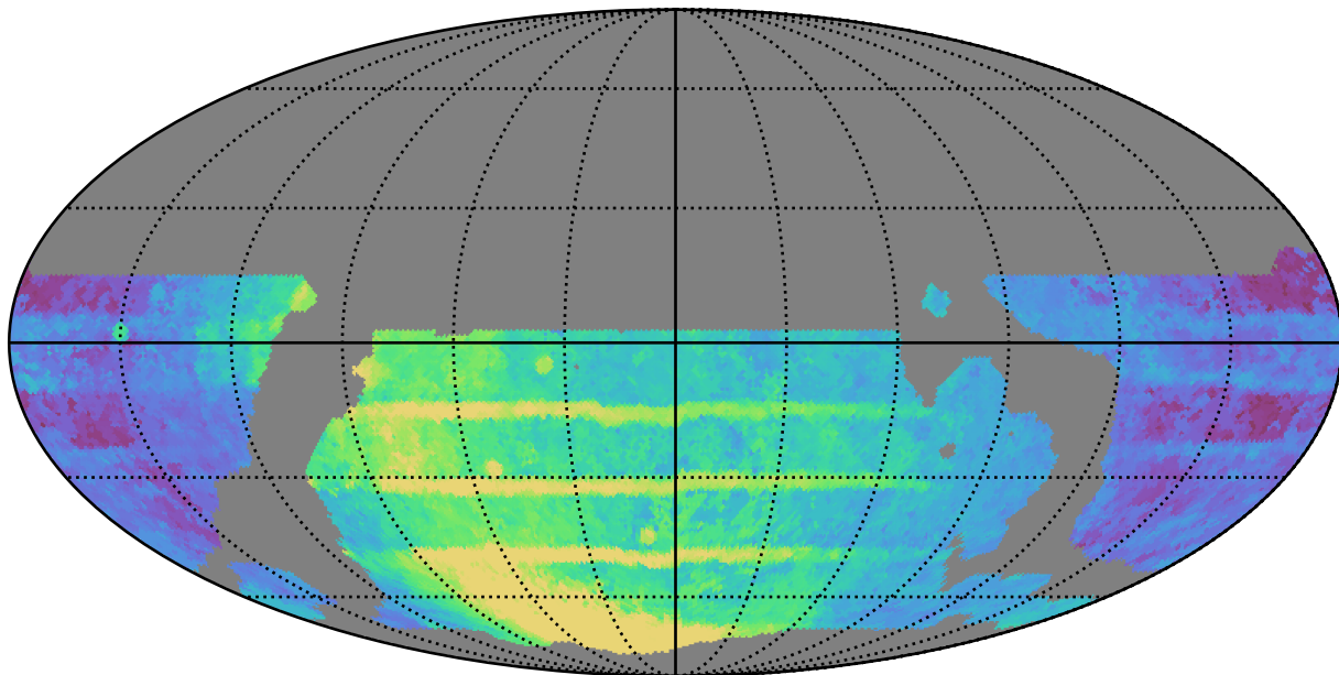
weather_cloudso18v3.4_10yrs WFD all bands: Median Season Length
