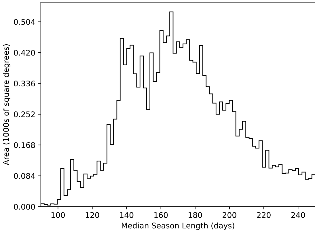
weather_cloudso18v3.4_10yrs WFD all bands: Median Season Length
