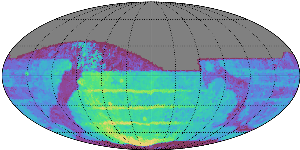
weather_cloudso18v3.4_10yrs All sky z band: Median Season Length
