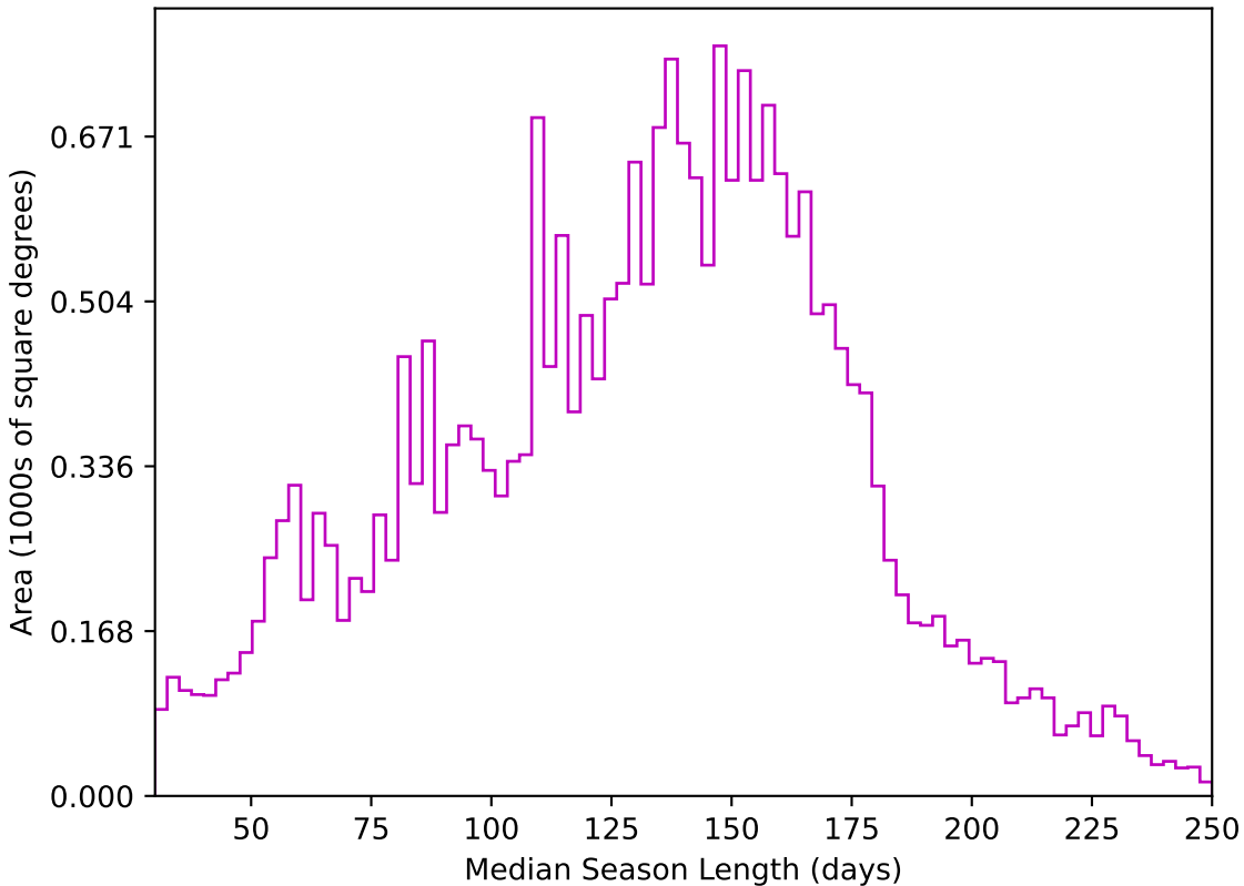
weather_cloudso18v3.4_10yrs All sky z band: Median Season Length
