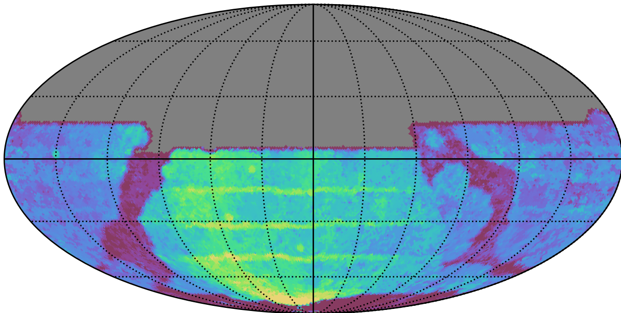
weather_cloudso18v3.4_10yrs All sky y band: Median Season Length
