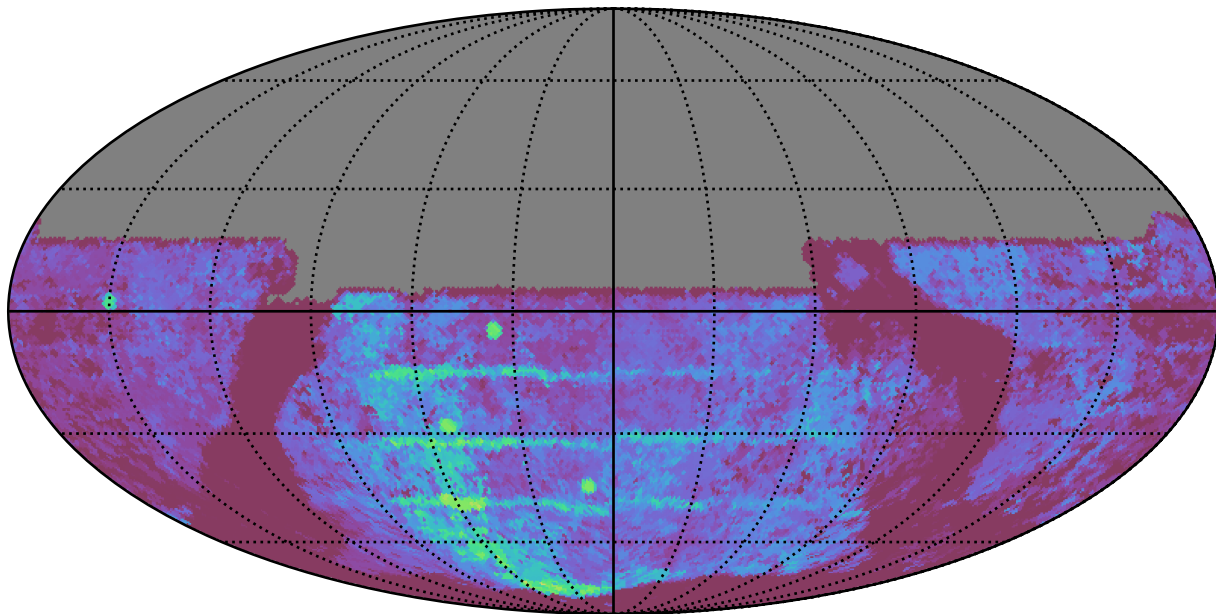
weather_cloudso18v3.4_10yrs All sky u band: Median Season Length
