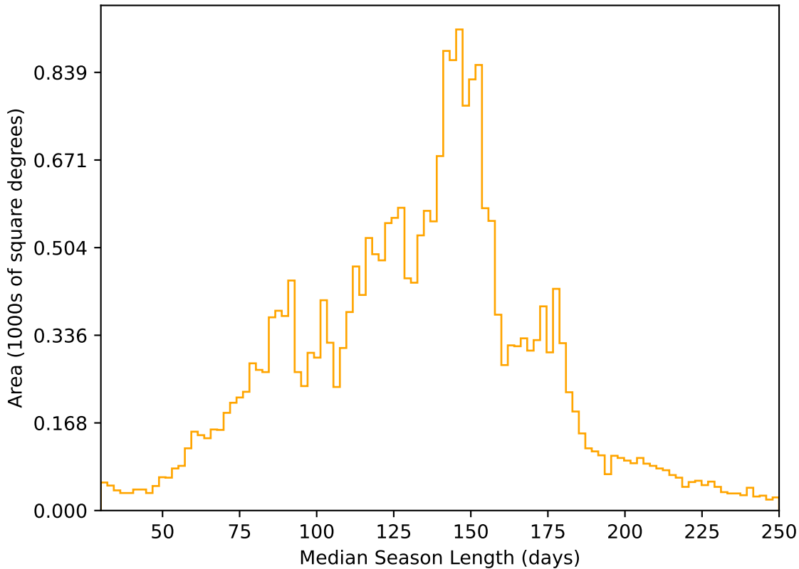
weather_cloudso18v3.4_10yrs All sky r band: Median Season Length
