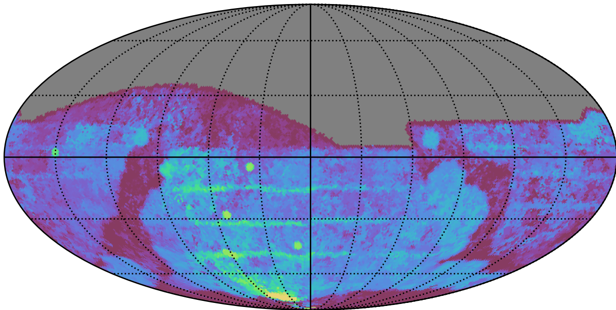
weather_cloudso18v3.4_10yrs All sky g band: Median Season Length
