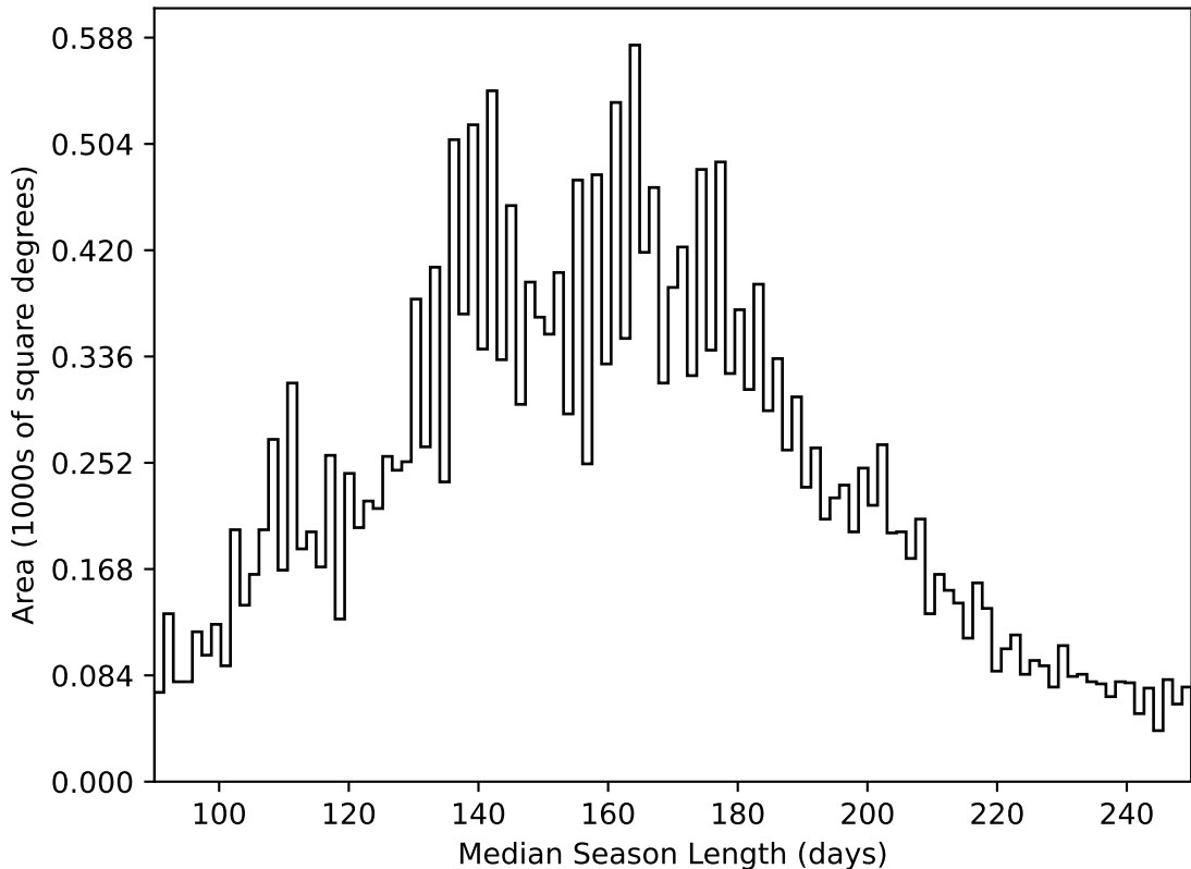
weather_cloudso18v3.4_10yrs All sky all bands: Median Season Length
