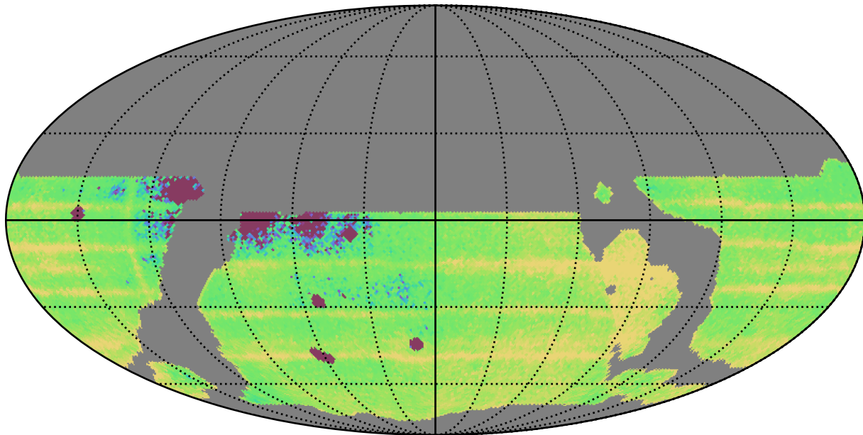
weather_cloudso18v3.4_10yrs WFD: Median Intra-Night Gap
