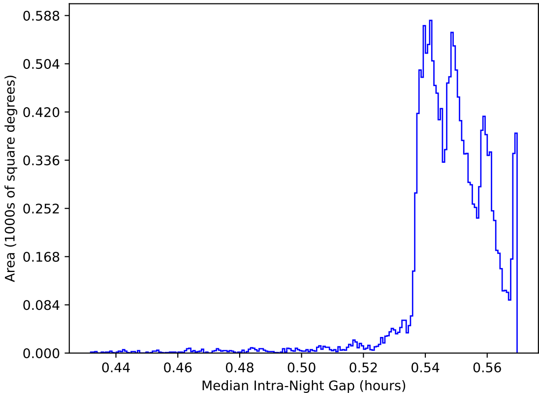
weather_cloudso18v3.4_10yrs WFD: Median Intra-Night Gap
