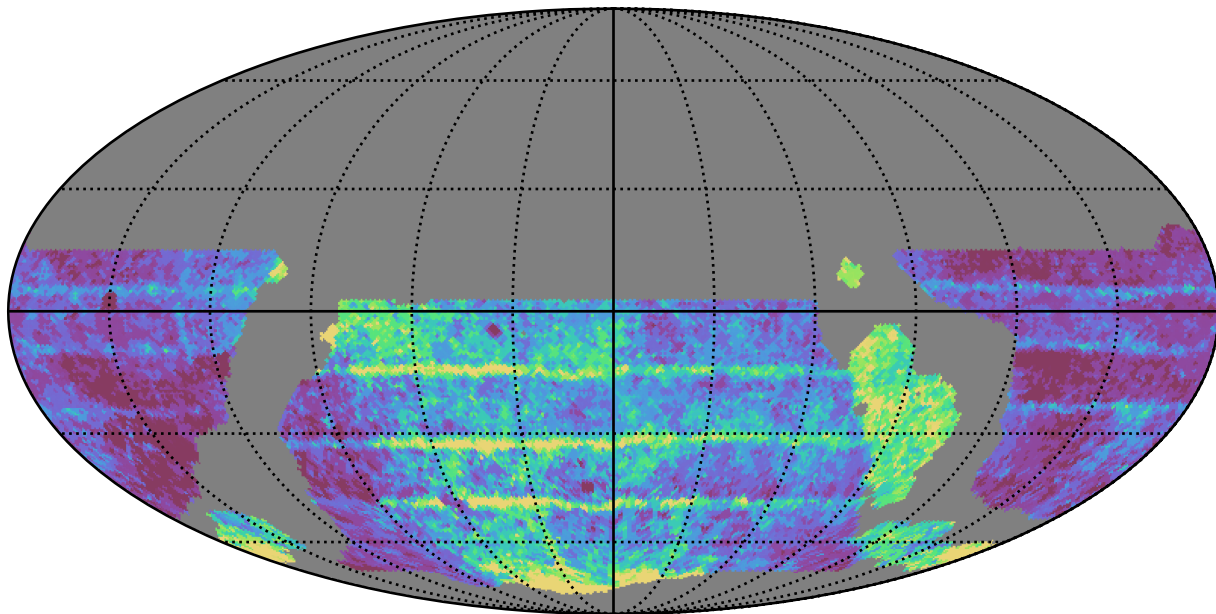
weather_cloudso18v3.4_10yrs WFD z band: Median Inter-Night Gap
