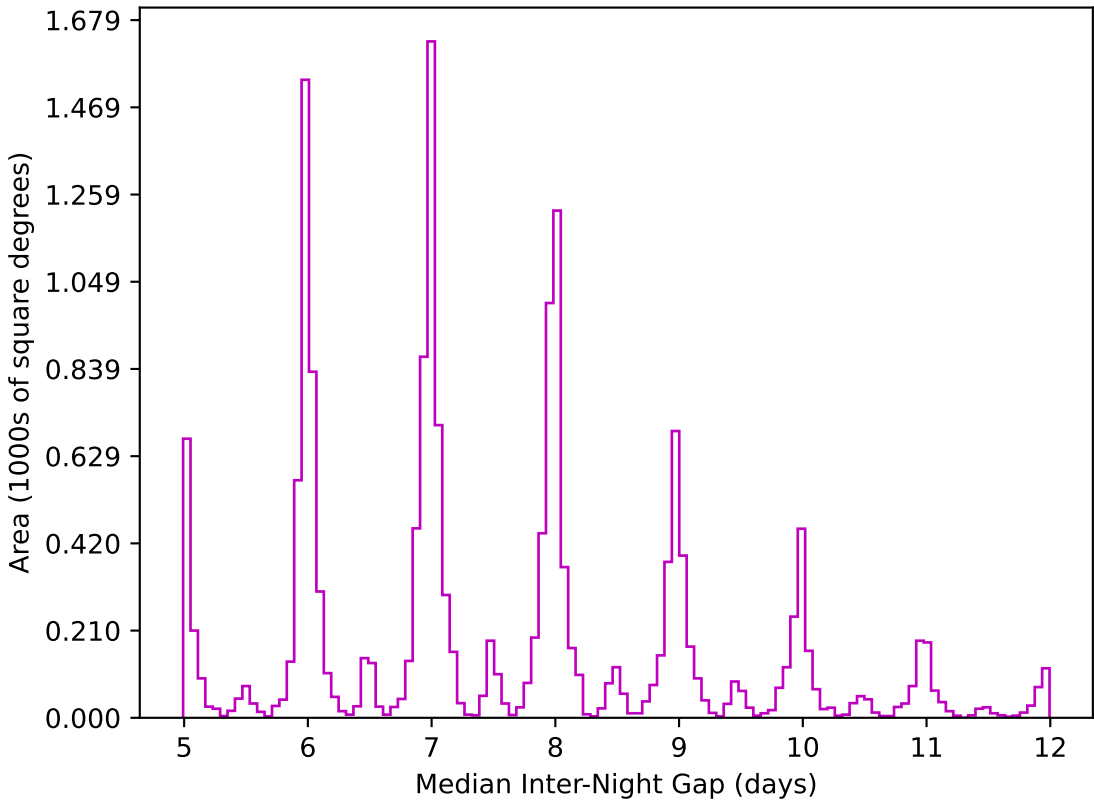
weather_cloudso18v3.4_10yrs WFD z band: Median Inter-Night Gap
