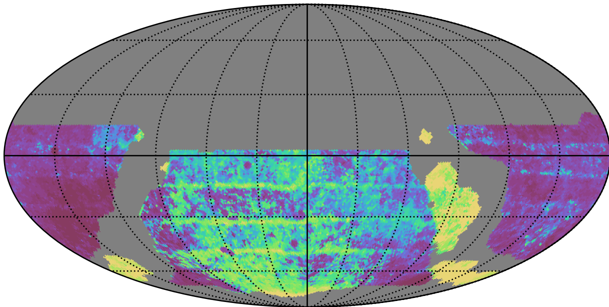
weather_cloudso18v3.4_10yrs WFD y band: Median Inter-Night Gap
