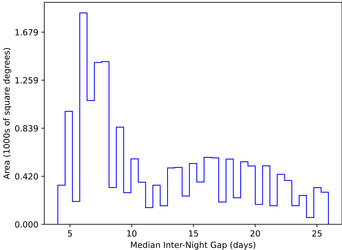
weather_cloudso18v3.4_10yrs WFD y band: Median Inter-Night Gap
