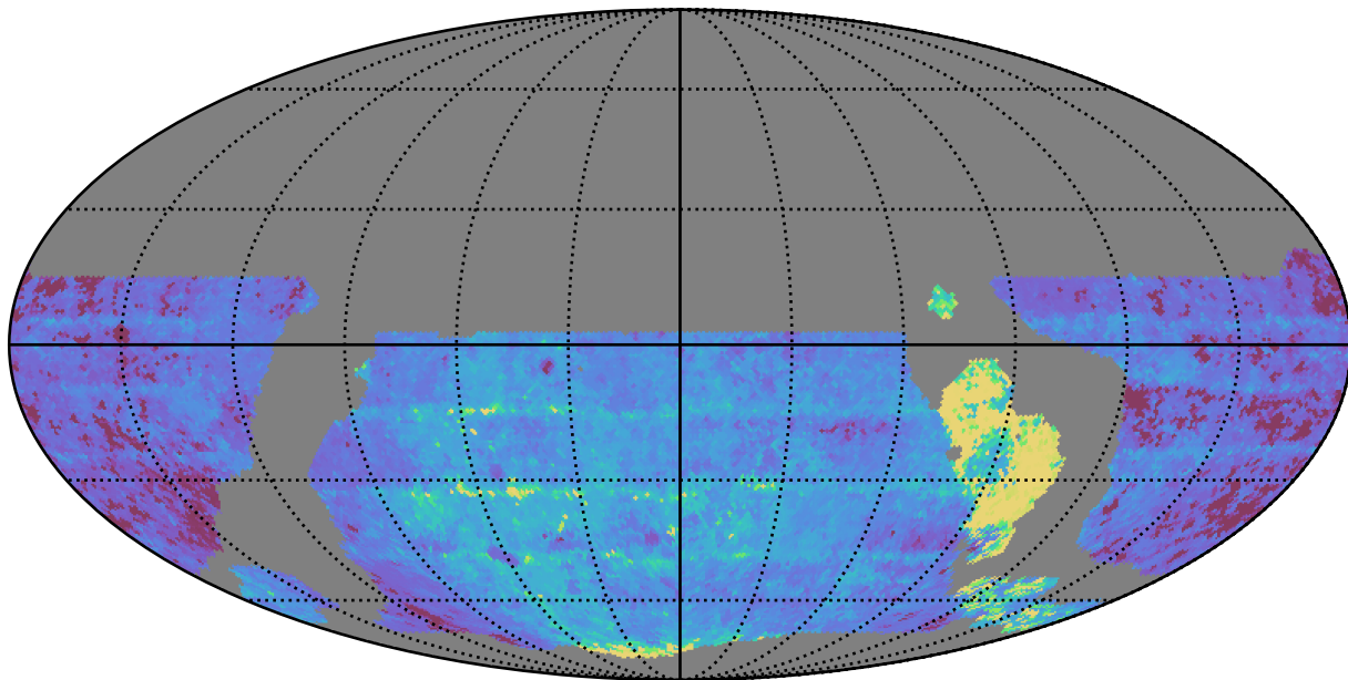
weather_cloudso18v3.4_10yrs WFD u band: Median Inter-Night Gap
