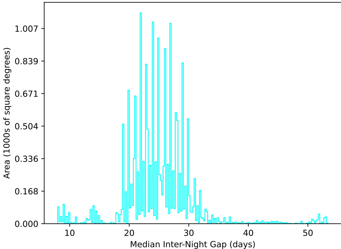
weather_cloudso18v3.4_10yrs WFD u band: Median Inter-Night Gap
