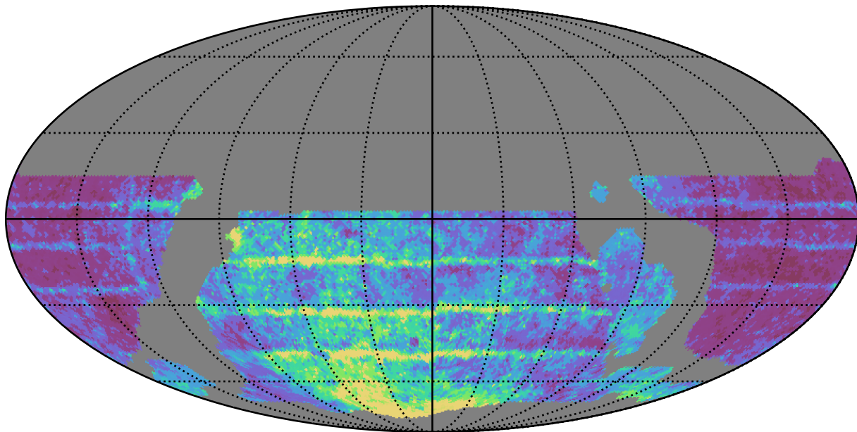
weather_cloudso18v3.4_10yrs WFD r band: Median Inter-Night Gap
