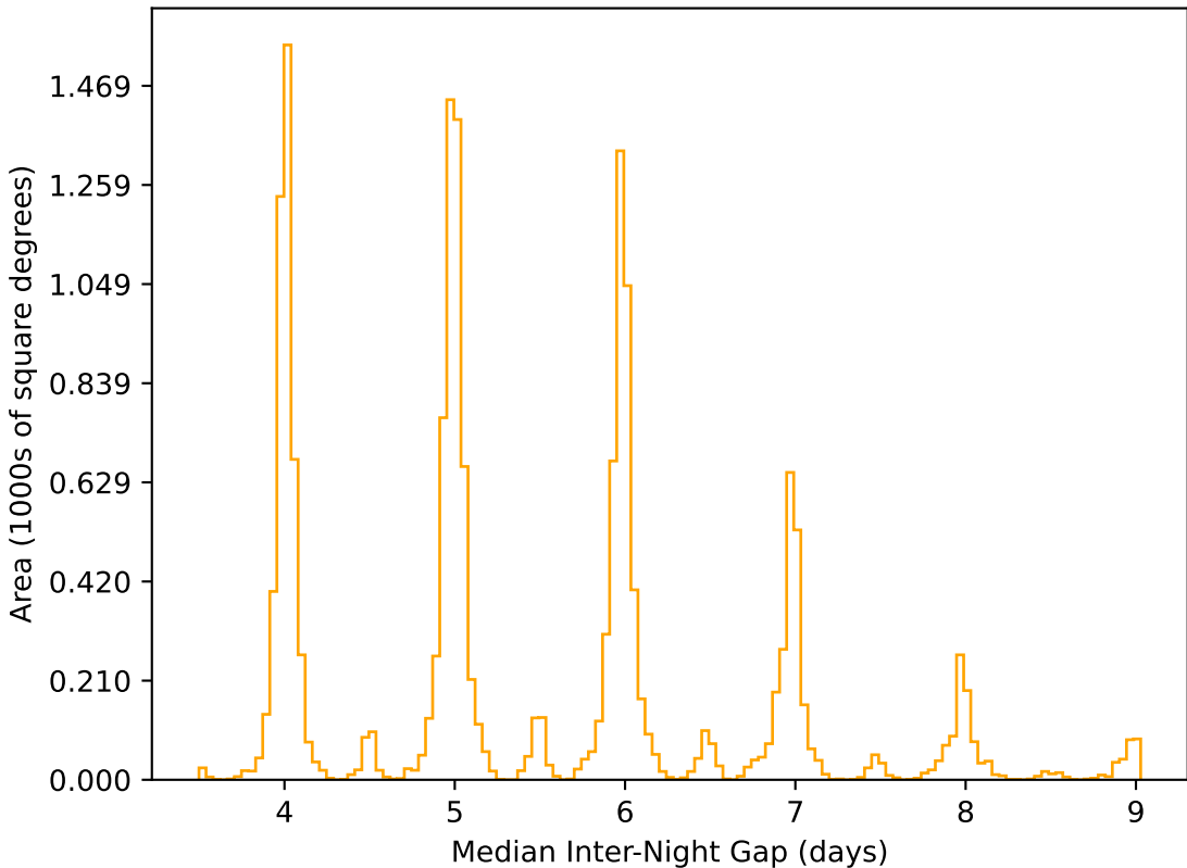
weather_cloudso18v3.4_10yrs WFD r band: Median Inter-Night Gap
