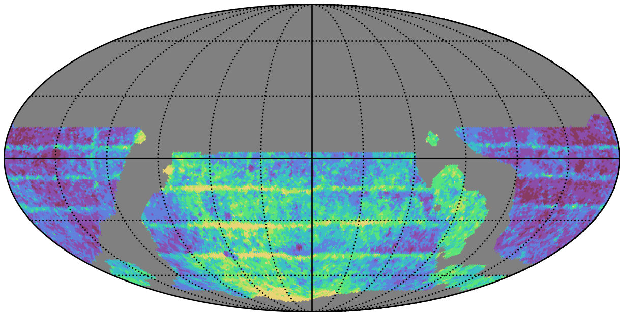
weather_cloudso18v3.4_10yrs WFD i band: Median Inter-Night Gap
