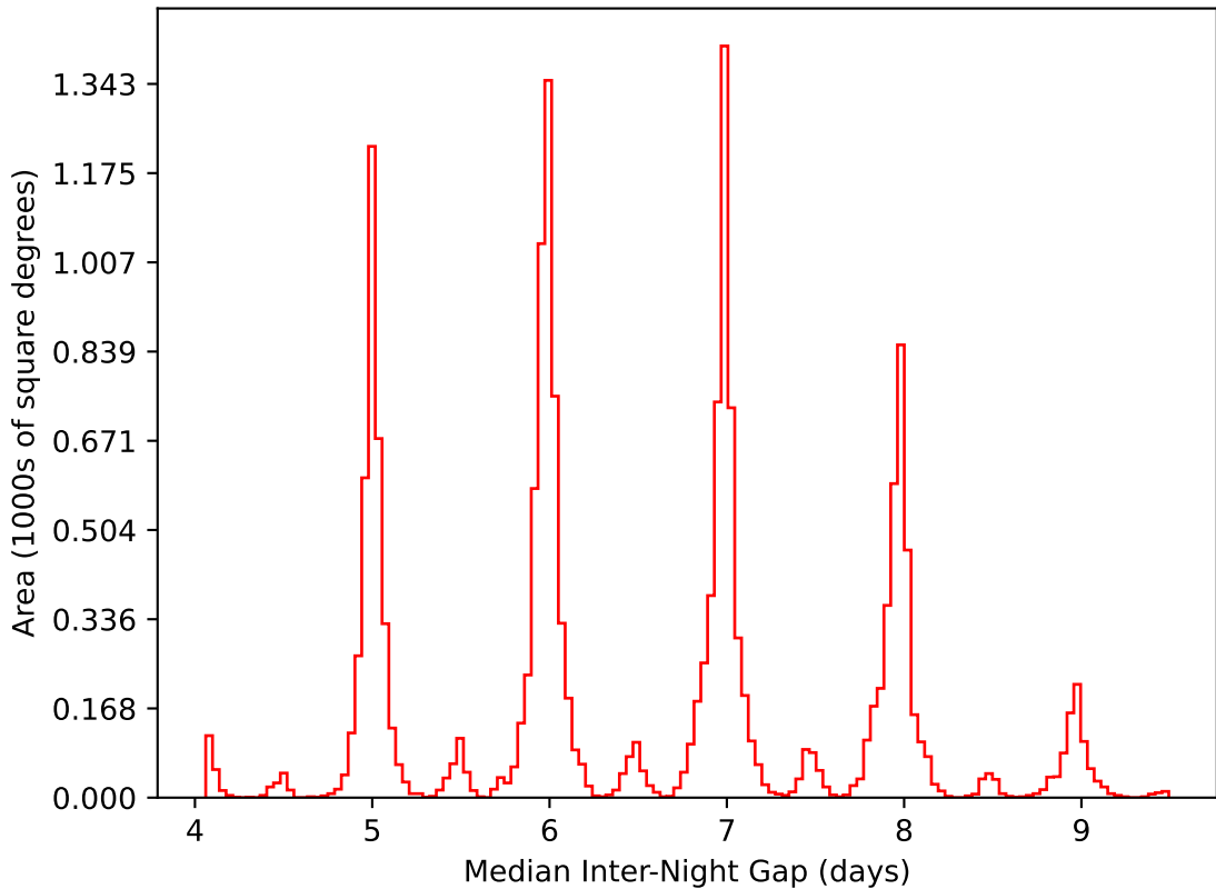
weather_cloudso18v3.4_10yrs WFD i band: Median Inter-Night Gap
